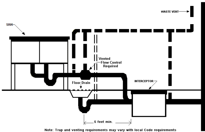
Figure A1.5.8- Interceptor Serving Sink protected from waste with Floor drain
