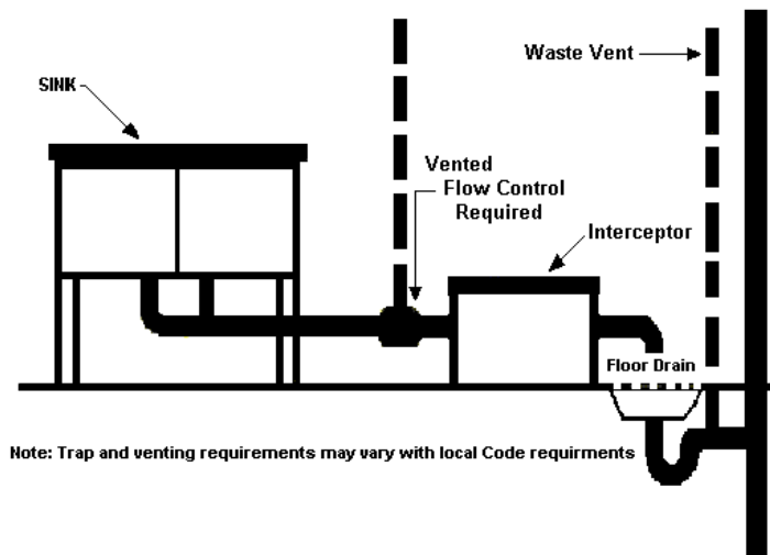
Figure A1.5.12- Interceptor Serving Sink with Indirect waste
